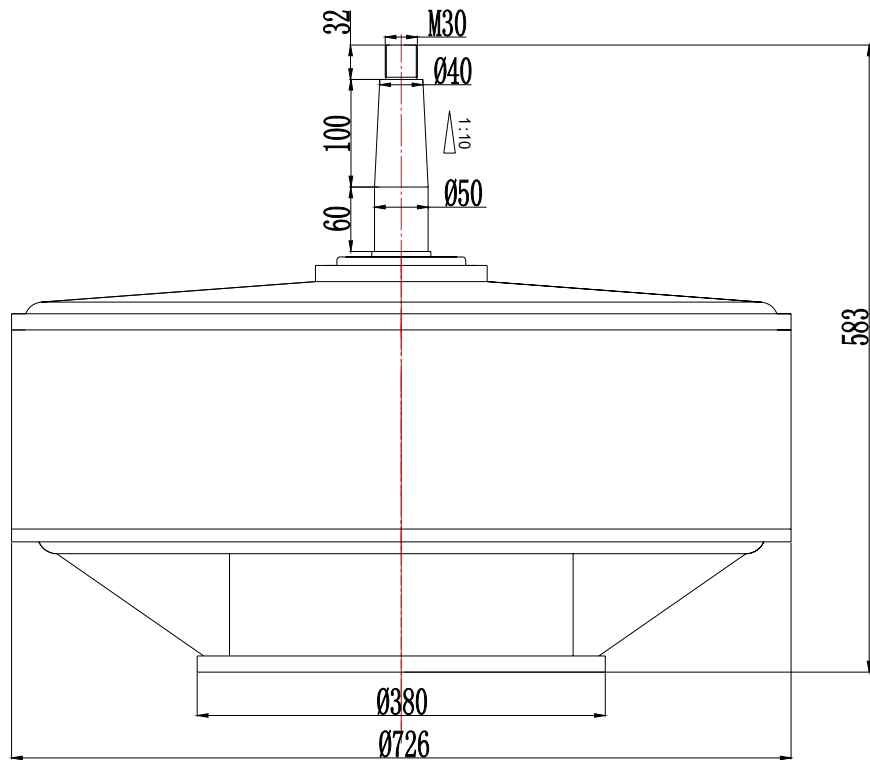
5KW Vertical Axis Wind Generator Dimensions
